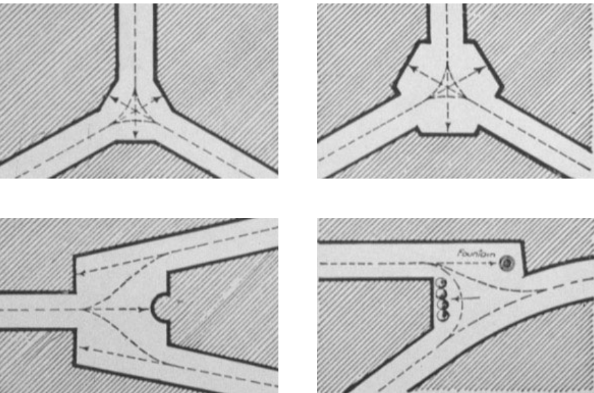
FROM THE TEXTBOOKS (1909): TRADITIONAL INTERSECTIONS, DESIGNED TO CREATE MEMORABLE PLACES, ARE OFTEN OUTLAWED BY SUBDIVISION ORDINANCES.
